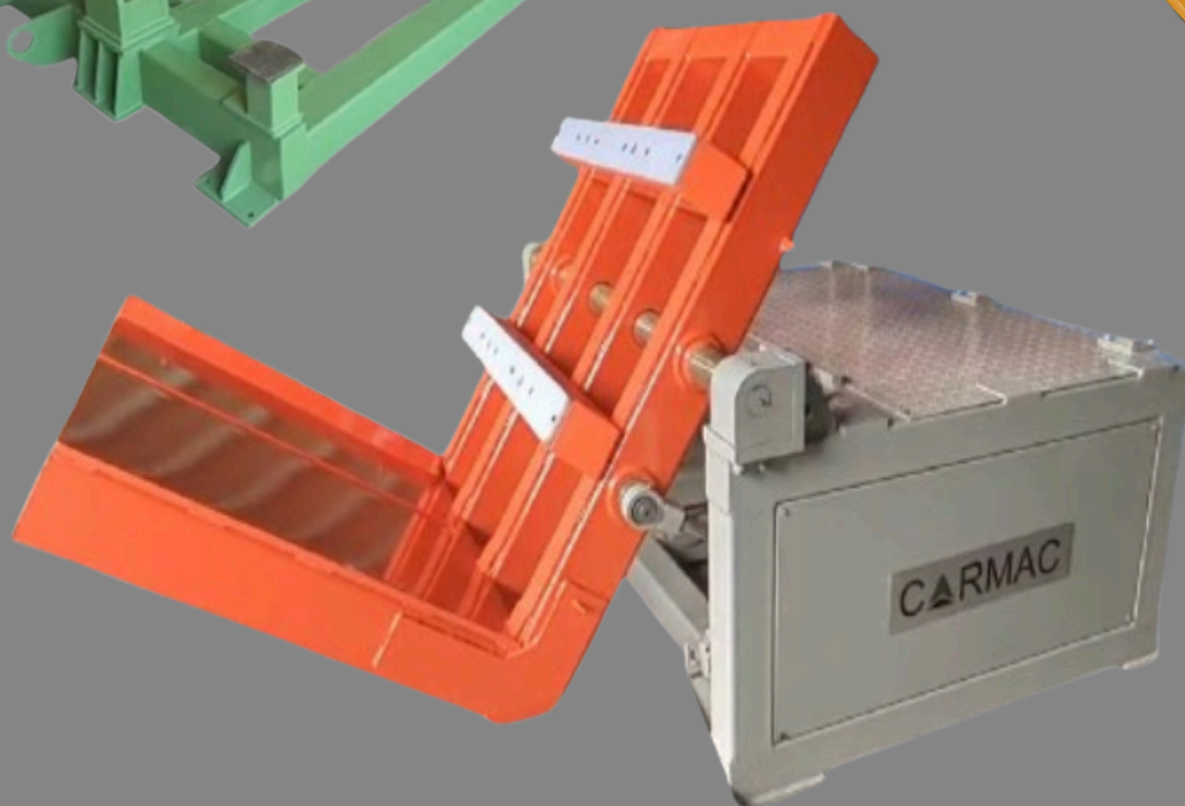
Hydraulic Coil Tilter – 1 Ton
